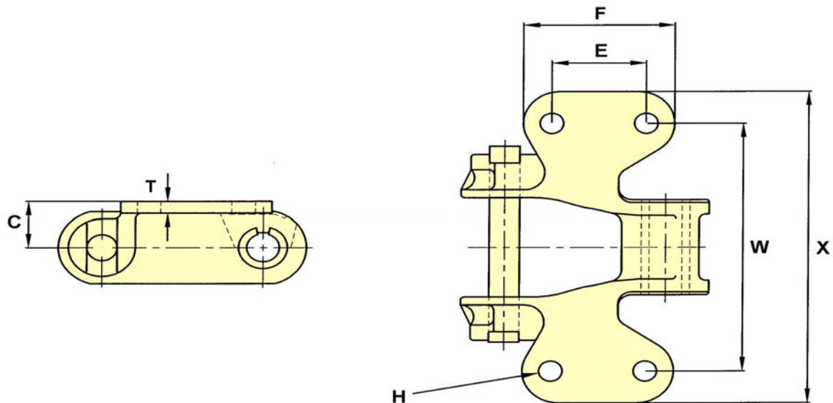
DRAWING NO. 130
