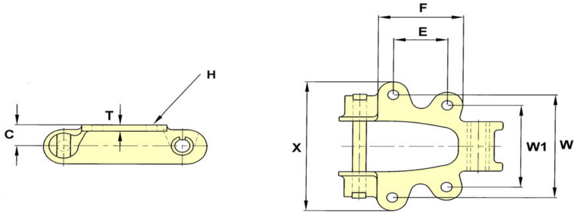
DRAWING NO. 161
