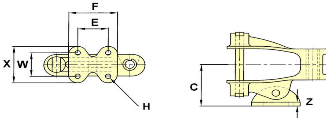
DRAWING NO. 157
