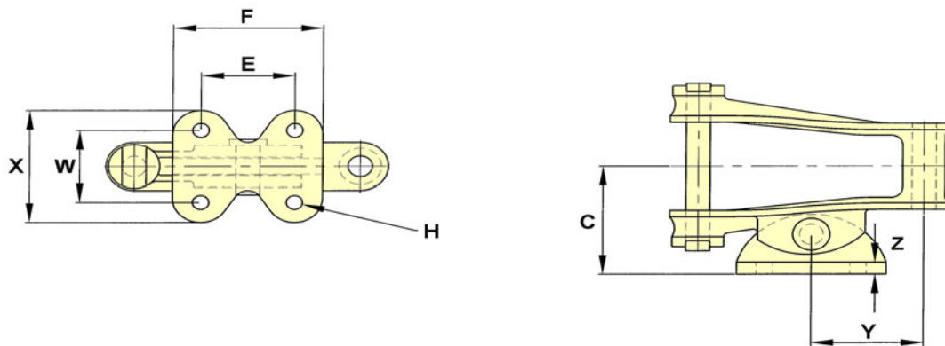
DRAWING NO. 207
