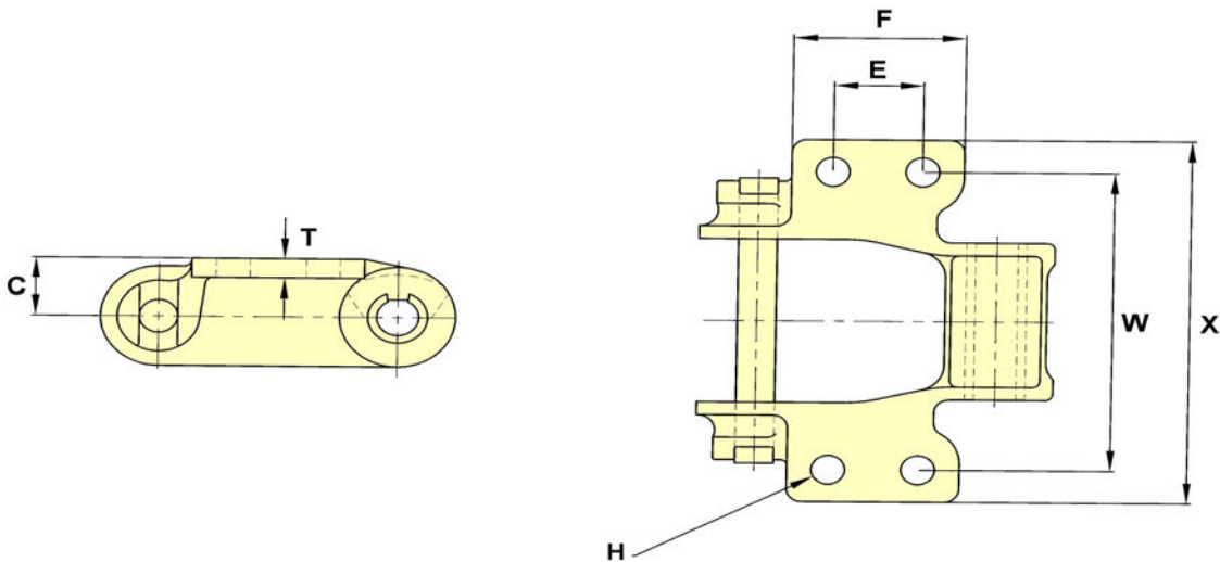
DRAWING NO. 162
