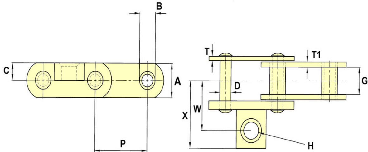
DRAWING NO. 184
