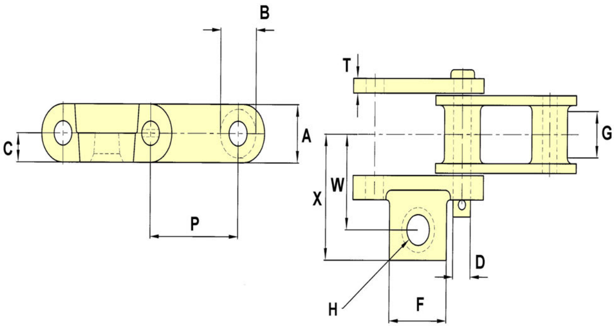
DRAWING NO. 141
