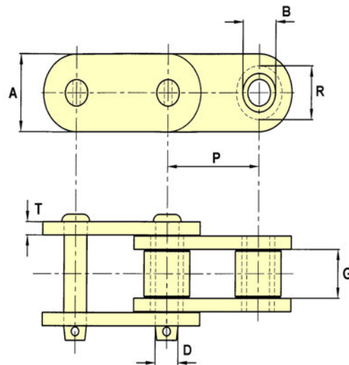
DIRECTION OF TRAVEL ↔ STYLE 1 - STRAIGHT SIDEBAR
