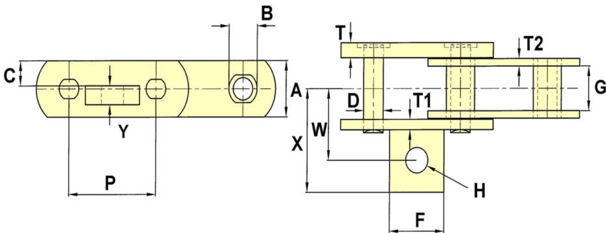
DRAWING NO. 259
