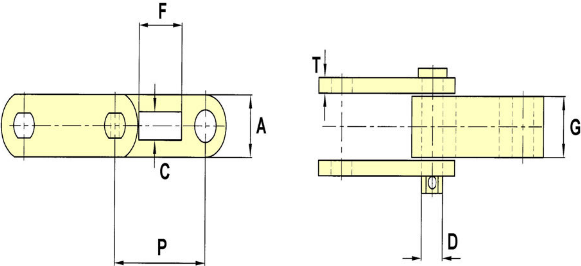
DRAWING NO. 182
