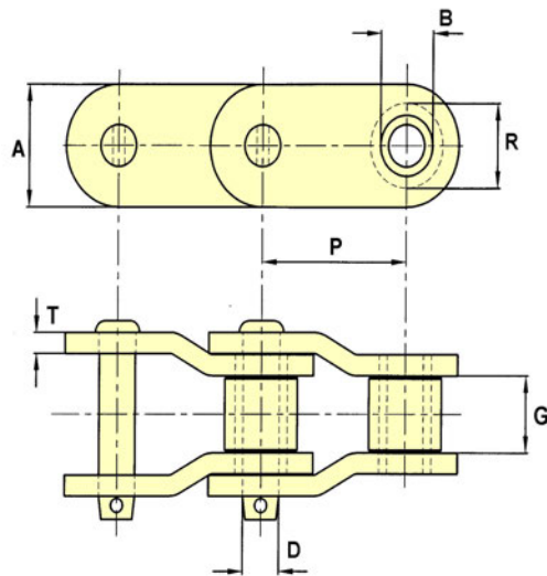
DIRECTION OF TRAVEL → STYLE 2 - CRANKED SIDEBAR
