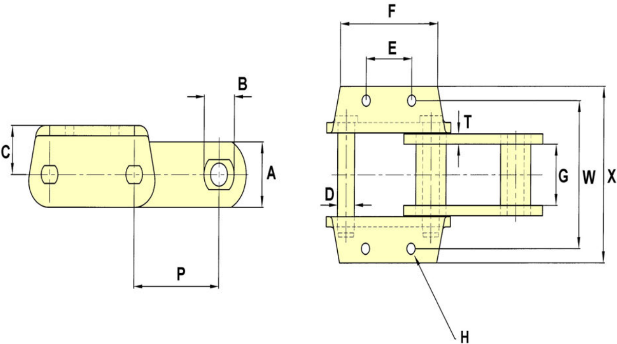
DRAWING NO. 159
